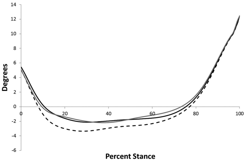
Figure 4. Frontal plane angle at the ankle for each of the conditions (control condition in black solid, lateral wedge condition in black dashed, lateral wedge plus arch support condition in gray solid). Eversion is negative. There were no significant differences between the control condition and either orthotic, but the ankle eversion angle peak was significantly higher in the lateral wedge condition than the lateral wedge plus arch support condition. Frontal plane excursion was significantly reduced with the use of the lateral wedge plus arch support compared to the control condition and the lateral wedge.
